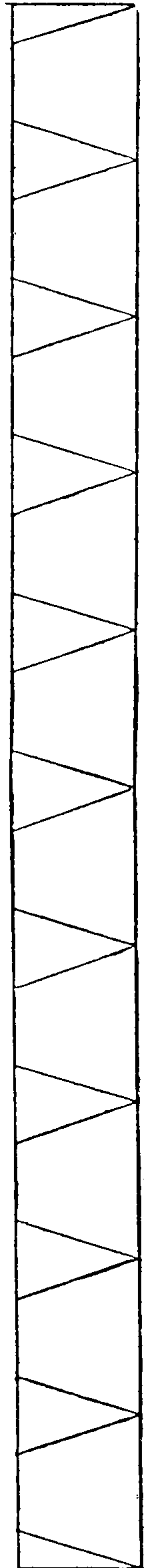
The analysis of the decagon.
