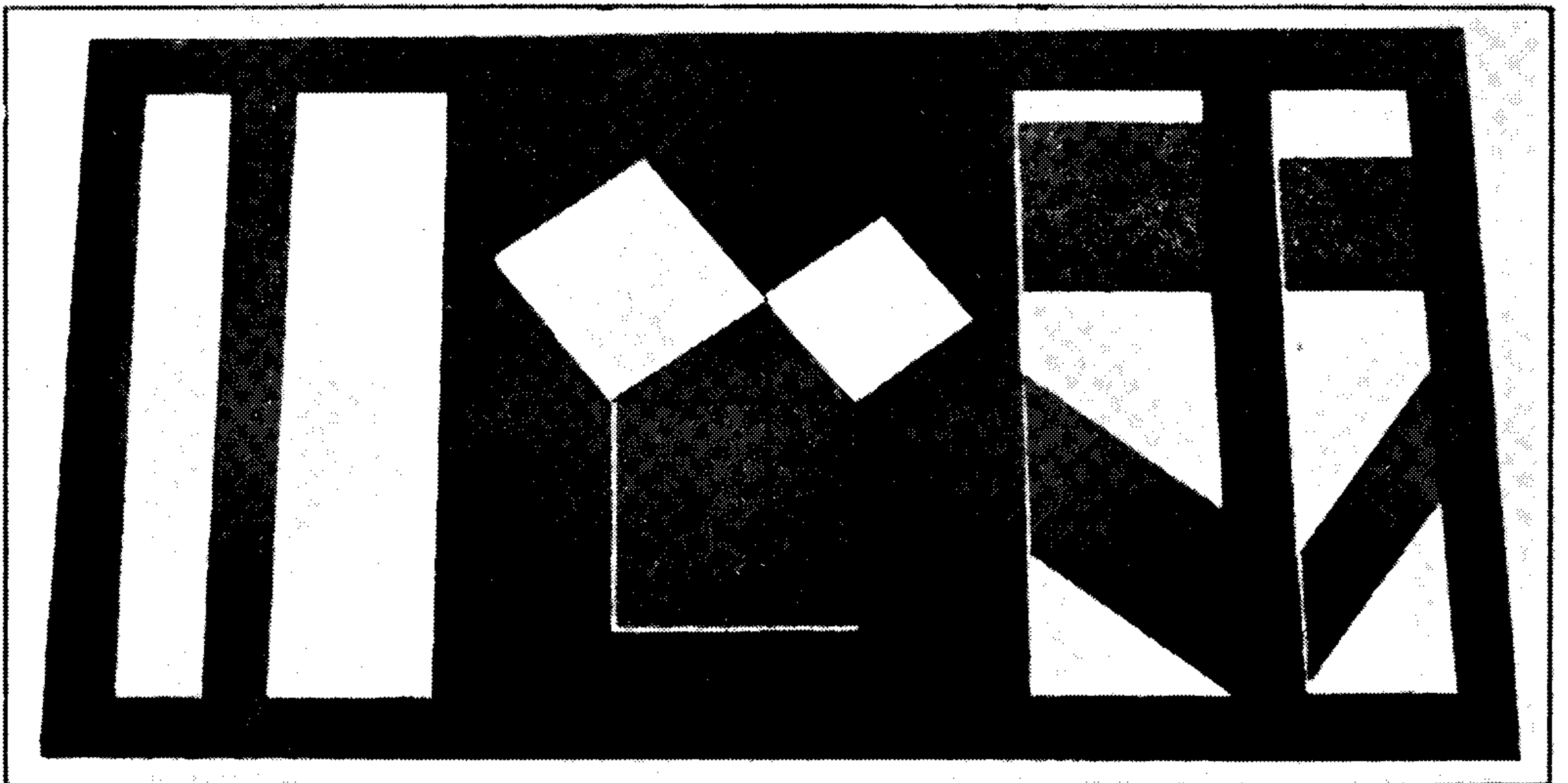
Showing that the two rhomboids are equal to the two squares.
