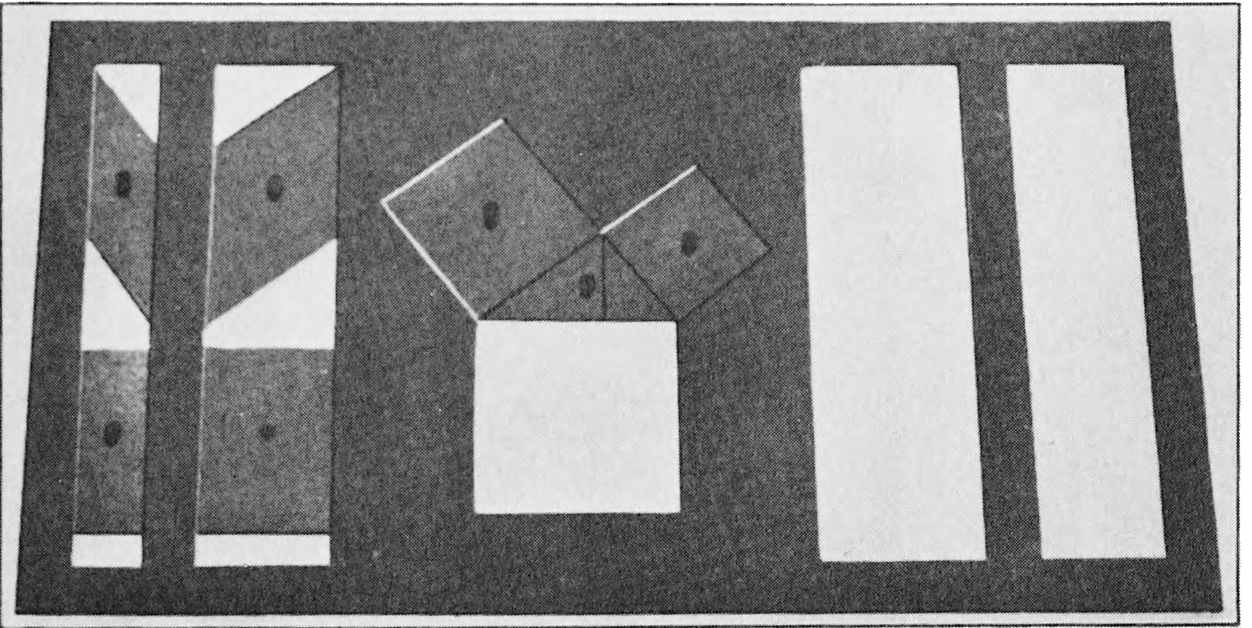
Showing that the two rhomboids are equal to the two rectangles.
